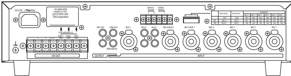
Rear View
